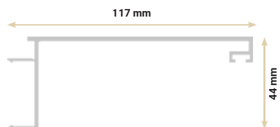
8 Capot de support Support cover
