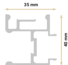
9 Profil d'éclairage LED LED Lighting Profile
