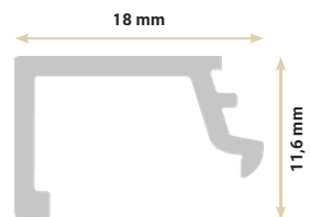
6 Pareclose verre simple Cover simple glass
